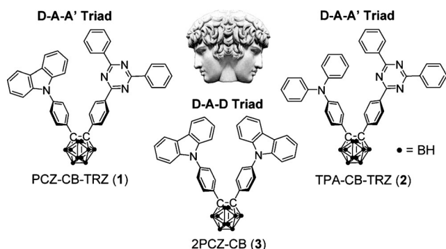
Figure 1. Structural formulae of Janus carboranes 1–3 (Janus is a Roman god and is depicted having two faces).
